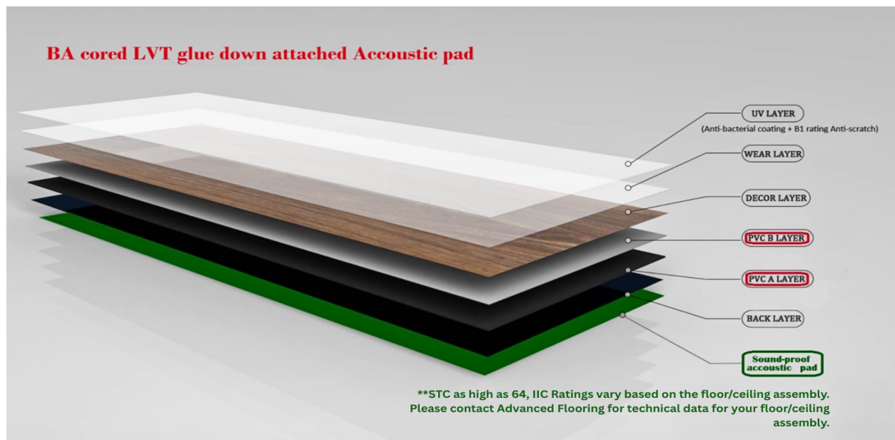
BA Cored LVT Glue Down — Attached Acoustic Pad Construction
